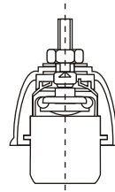
Rocking feature in non rotating Bobbin Holder
